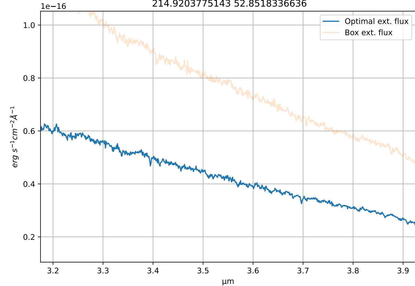
jw01345013 GRISM 18859 AB:-8.95 214.9203775143 52.8518336636
