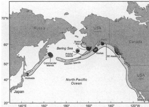
FIG. 1.—Distribution of harbor seals in the Pacific Ocean. Centers of abundance are shaded, and boundaries of the currently recognized management stocks within Alaska are indicated by dashed lines. PWS, Prince William Sound.
