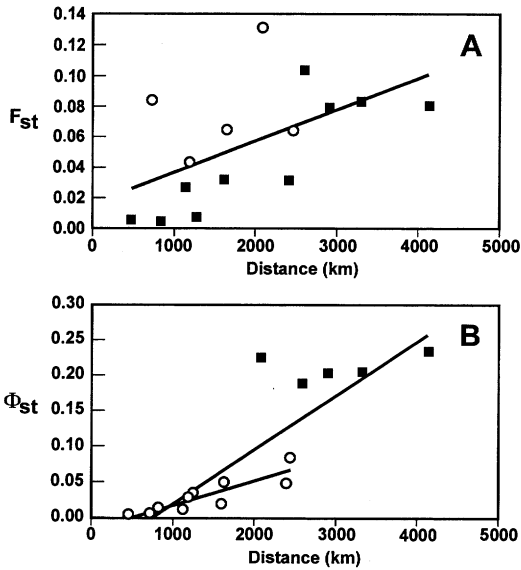
FIG. 4.—The relationship between genetic and geographic distance in harbor seals across the North Pacific Ocean from the Commander Islands to Southeast Alaska. A) Relationship between frequency-based F_{ST} and minimum swim distance ( r^2 = 0.317 , P = 0.069 ). Pairwise comparisons involving the Pribilof Islands are represented by open circles. B) Relationship between distance-based \Phi_{ST} and minimum swim distance ( r^2 = 0.729 , P = 0.00001 ). A regression of \Phi_{ST} on swim distance for the Alaska regions only (represented as open circles) is also presented ( r^2 = 0.775 ).
