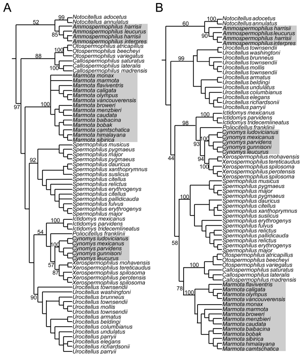
FIG. 2.—Phylogeny of Marmotini proposed by Herron et al. (2004) based on analyses of complete sequences of the cytochrome- b gene. Harrison et al. (2003) presented very similar results. Multiple terminal branches representing the same taxon have been collapsed for simplification in some cases, and some identifications have since been modified. The shaded taxa represent the 3 genera that have not been traditionally recognized in Spermophilus . A) Maximum parsimony: “Strict consensus of all 208 equally optimal trees based on unweighted maximum parsimony search” (Herron et al. 2004:1022). Bootstrap percentages for nodes of taxonomic interest (generic and supergeneric) are shown following Herron et al. (2004). B) Bayesian analysis: “Majority rule consensus phylogram (with branch lengths averaged over all trees) resulting from Bayesian phylogenetic analysis using a GTR + G + I model of evolution” (Herron et al. 2004:1024). Posterior probabilities “estimated from a total of 4 million post-burn-in generations (from four independent runs)” are provided for nodes of taxonomic interest (generic and supergeneric) following Herron et al. (2004:1024).
