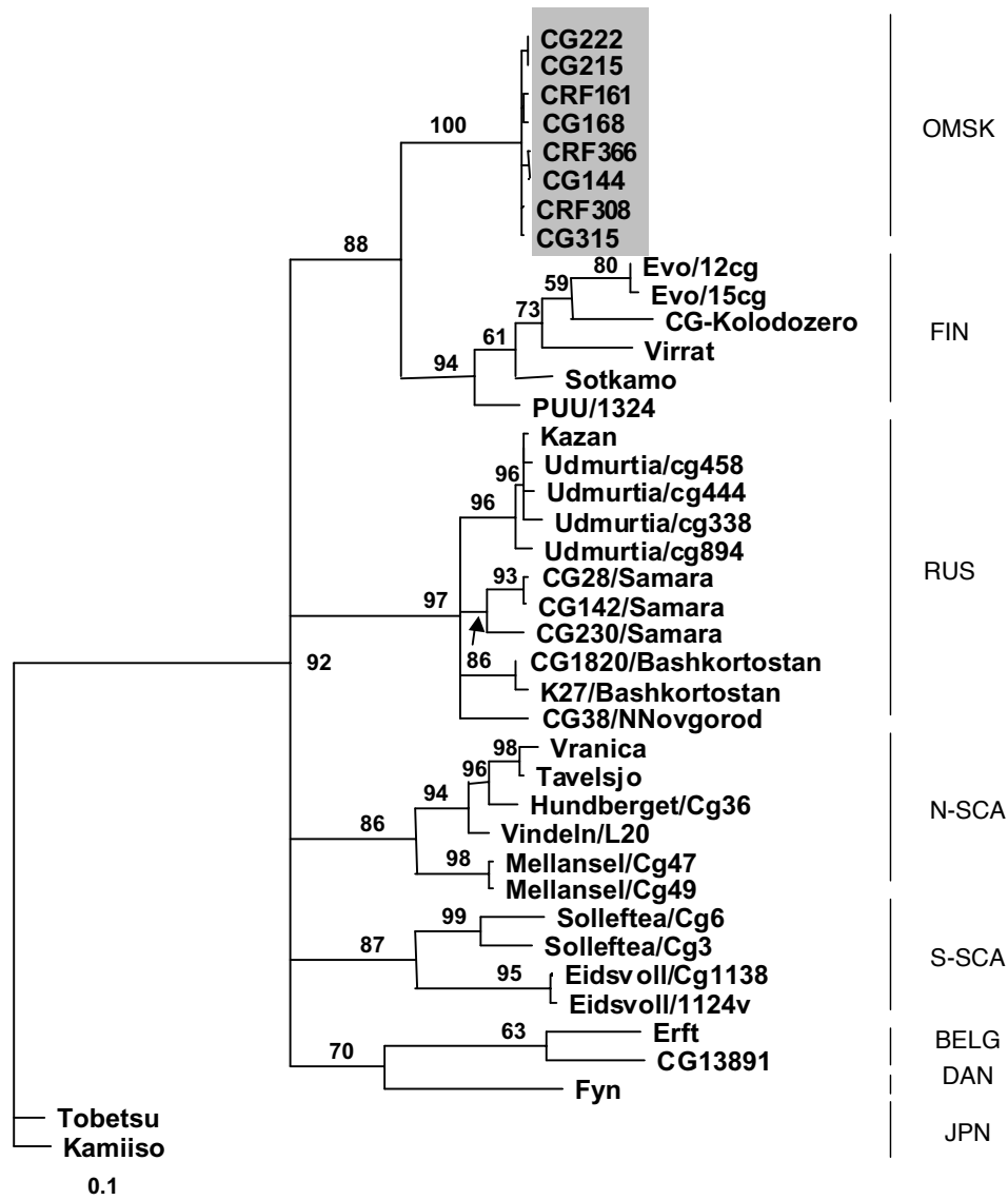
Fig. 2. Phylogenetic analysis based on partial sequences of the S-segment (630 nt), generated by maximum-likelihood method. Bootstrap values are expressed as percentages of the total number of replicates (10,000). PUU viruses originating from the Omsk region are indicated by shading. The S-segment sequences included PUU strains: Sotkamo (X61035), PUU/1324Cg/79 (Z46942), Evo/12Cg/93 (Z30702), Evo/15Cg/93 (Z30705), Virrat/25Cg/95 (Z69985), CG13891 (U22423), PUU/Cg-Erft (AJ238779), Fyn (AJ238791), VindelIn/L-20 (Z48586), Mellansel/Cg47/94 (AJ223374), Mellansel/Cg49/94 (AJ223375), Hunberget/Cg36/94 (AJ223371), Solleftea/Cg3/95 (AJ223376), Solleftea/Cg6/95 (AJ223377), Tavelsjo/Cg81/94 (AJ223380), Eidsvoll/1124v (AJ223368), Eidsvoll/Cg1138/87 (AJ223369), Vranica (U14137), CG-Kolodozero (AJ238789), CG1820/Ufa-83 (M32750), K27/Ufa-85 (L08804) Udmurtia/894Cg/91 (Z21497), Udmurtia/338Cg/92 (Z30708), Udmurtia/444Cg/88 (Z30706), Udmurtia/458Cg/88 (Z30707), Kazan (Z84204), Tobetsu-60Cr-93 (AB010731) Kamiiso-8Cr-95 (AB010730). Genetic lineages indicated by abbreviations on the right.
